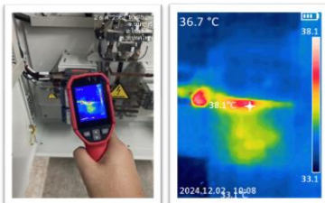
breaker Inverter No.1 38.1 °C
